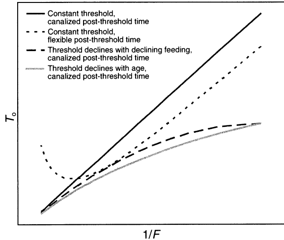
FIG. 1. Predicted relationships of time to oviposition ( T_o ) and inverse of daily food ration ( 1/F ) for four different models of development toward oviposition. All models postulate a threshold for initiation of the process of vitellogenesis and a post-threshold phase of development. The threshold may be fixed, as in hypotheses 1 and 2, or may show adaptive flexibility in response to food intake, as in hypotheses 3 and 4. Post-threshold development may be canalized and unresponsive to food intake, as in hypotheses 1, 3, and 4, or may show adaptive flexibility in response to food intake, as in hypothesis 2. See Relationships of development time and feeding rate for details.
