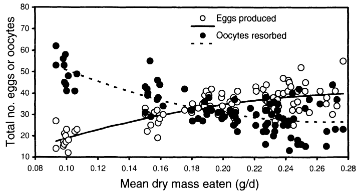
FIG. 3. Relationships of total number of eggs produced (laid + mature eggs retained) and oocytes resorbed to mean daily food intake. Quadratic regressions were significant for both total eggs (eggs = -7.3 + 314.1(F) - 519.3(F^2) ; R^2 = 0.62 , P < 0.0001 , N = 95 ) and oocytes resorbed (resorbed = 87.5 - 449.6(F) + 827.2(F^2) ; R^2 = 0.56 , P < 0.0001 , N = 88 ).
